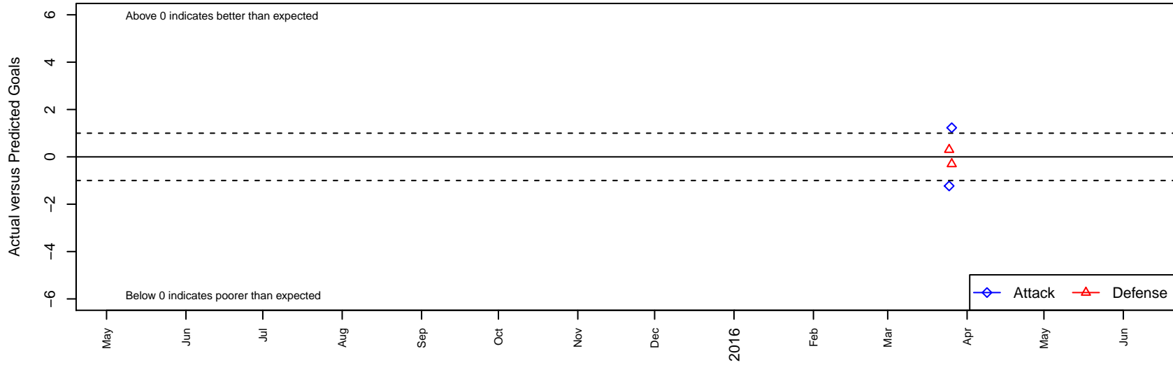
Coastal FC 1997B Dots are actual minus expected GF (blue circles) and GA (red triangles). Blue line is smoothed change in attack strength. Red is smoothed change in defense strength.
